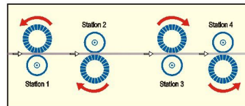
Surfacing.... Step by Step on Metal Strip
